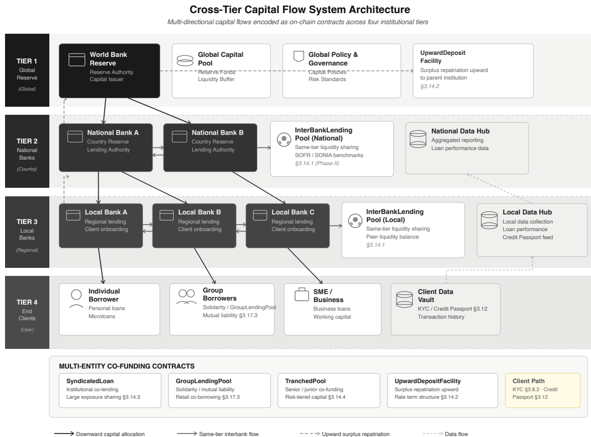
Figure 1.2: Cross-tier lending flow directions
