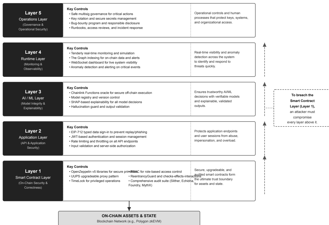
Figure 3.32: Five-layer defense-in-depth security architecture
