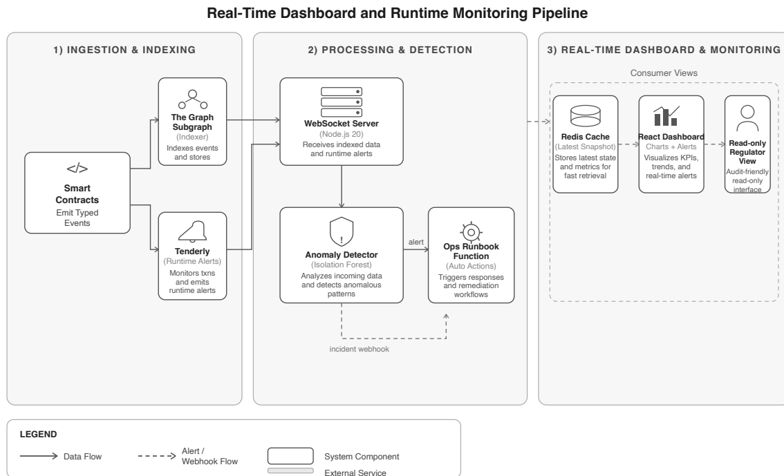
Figure 4.5: Real-time dashboard and runtime monitoring pipeline
