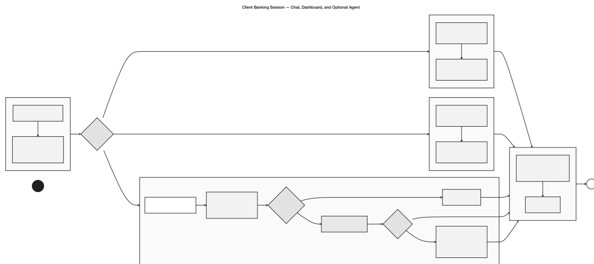
Figure 3.23: Client banking session activity flow
