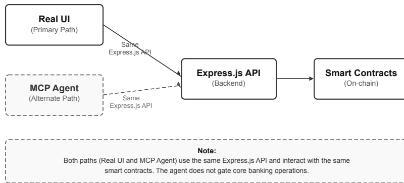
Figure 4.9: Optional conversational agent add-on
